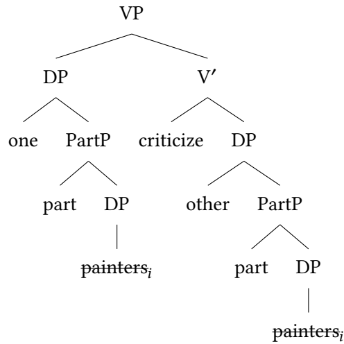
Figure 2: After ellipsis
